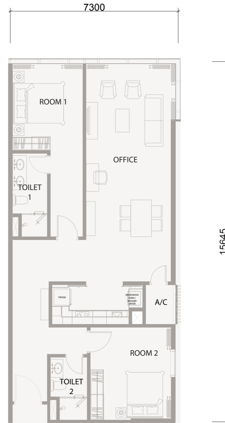
TYPE JH 1,195ft 2 (SQFT) 111.02m 2 (SQM)
